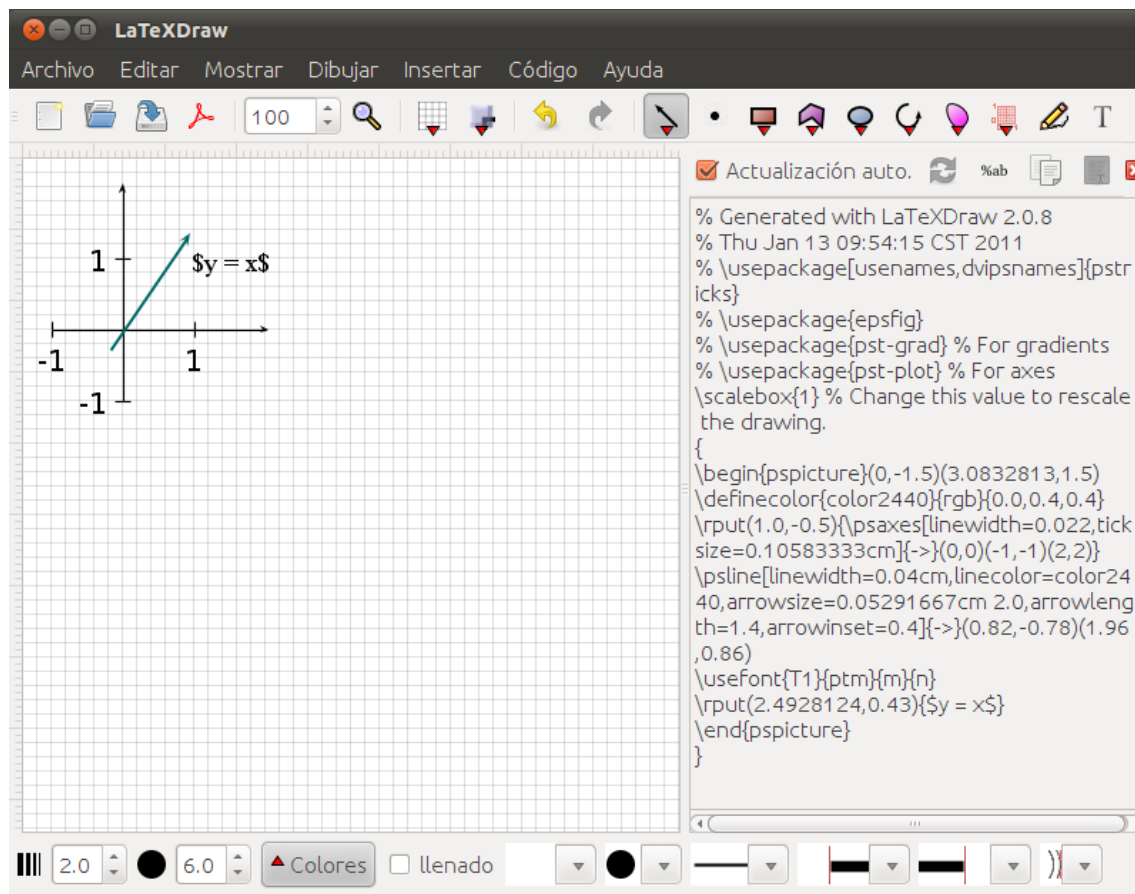
Figura 6.7 Editor LaTeXDraw
