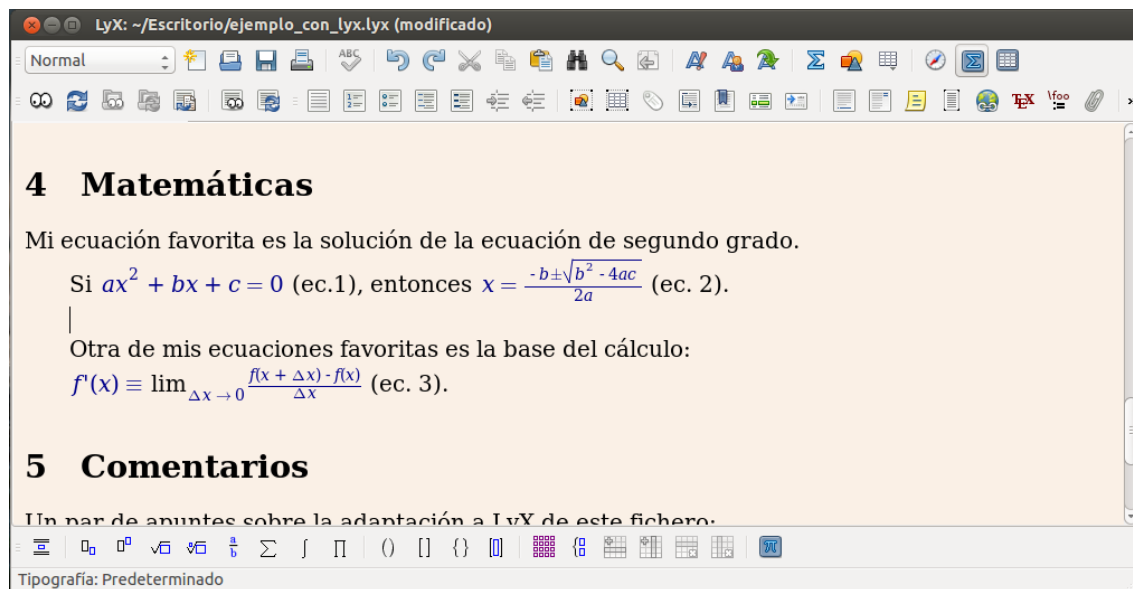
Figura C.4 Editor LyX
